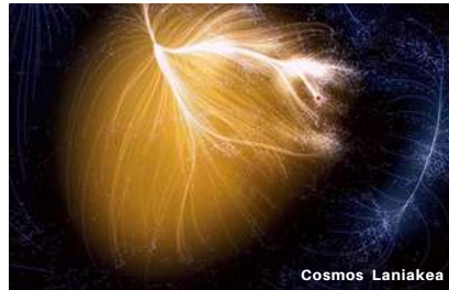
Cosmos Laniakea
